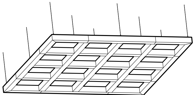
③ PERSPECTIVE VIEW
