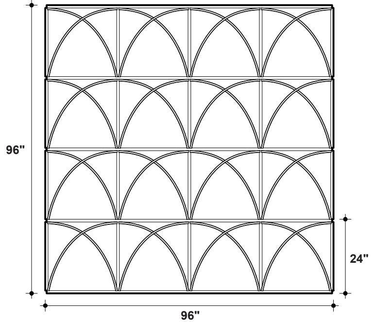
① BOTTOM VIEW
