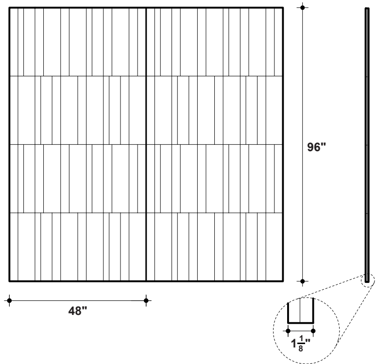
① FRONT & SIDE VIEW
