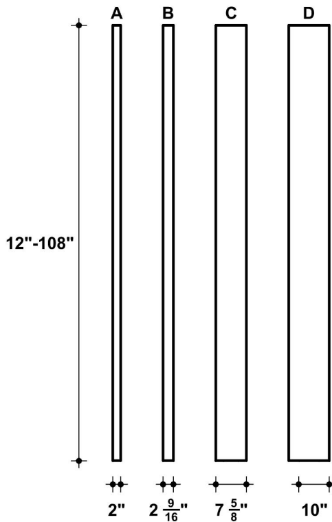
① FRONT VIEW
