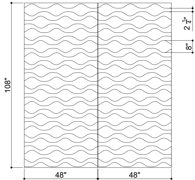
① FRONT VIEW
